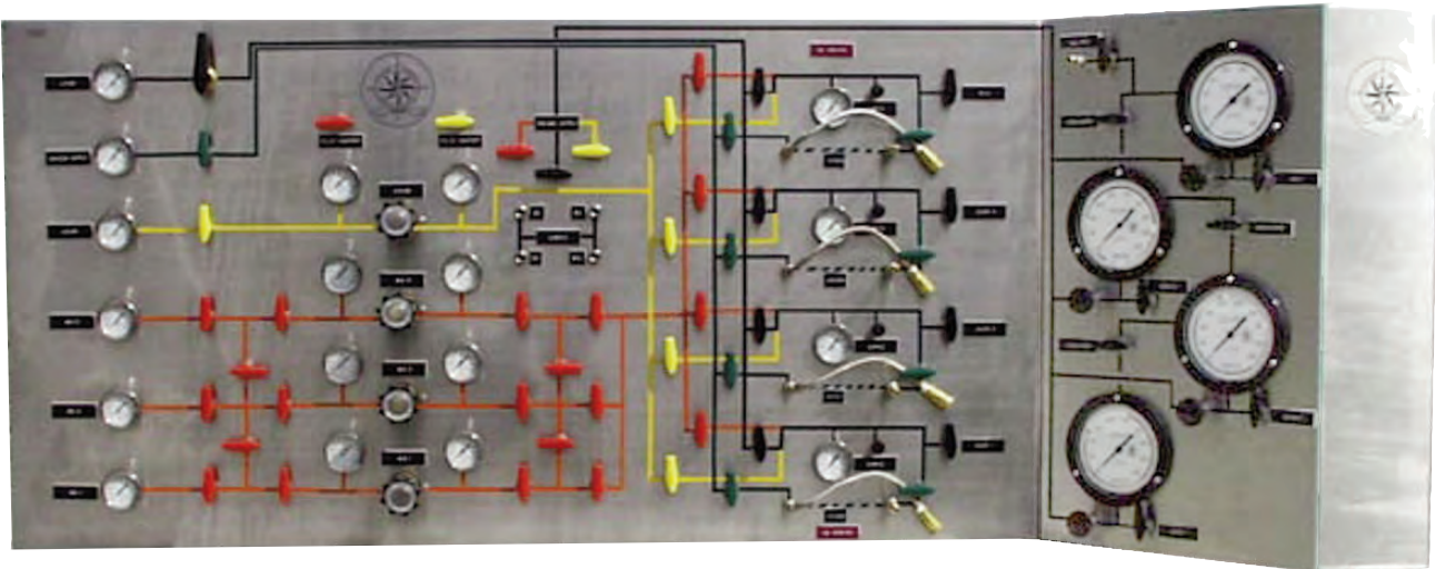
Gas Rack, Panel Mount
