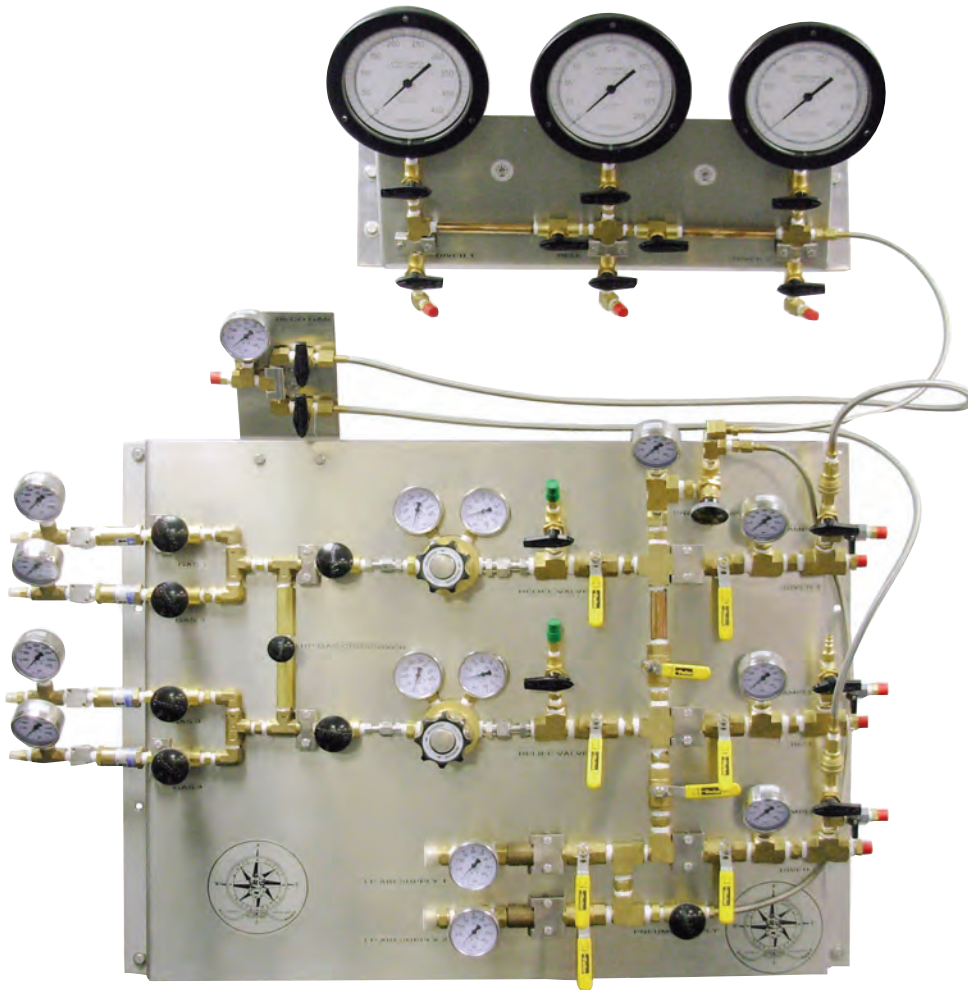
Gas Rack, Wall Mount Our Stock System GAS RACK 1B
